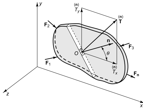
Fig. 4.12 Stress vector acting at point O on a plane whose normal is \mathbf{n} for a body subjected to plane stress
