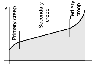
Fig. 5.47 Creep curve
