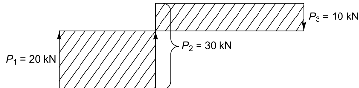
Fig. 2.4(c) Axial force diagram for Example 2.3(b)
