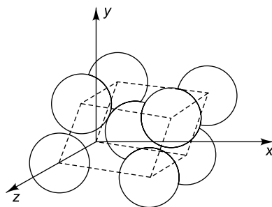
Fig. 5.25 An anisotropic crystal structure
