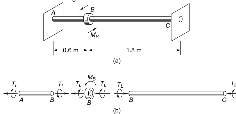
Fig. 6.24 Example 6.5. Limit analysis of a statically indeterminate torsion member
