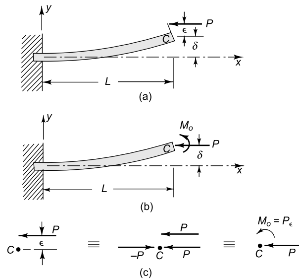
Fig. 9.13 Flexible column held in equilibrium by (a) a longitudinal compressive force P with eccentricity \epsilon and (b) the same compressive force P plus an end moment M_o . The equivalence of the two loadings is shown in (c)
