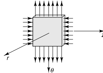
Fig. 5.33 State of stress in cylinder wall of Fig. 5.28(a) when \sigma_\theta and \sigma_z determine the maximum shear stress
