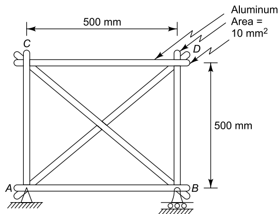
Fig. 2.16(a) Example 2.10(b)
