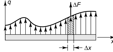
Fig. 3.7 Distributed load of intensity q
