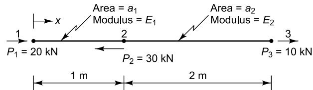
Fig. 2.4(a) Example 2.3(b)
