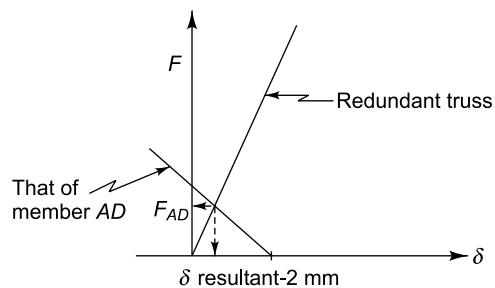
Fig. 2.16(b) Plot of force vs displacement
