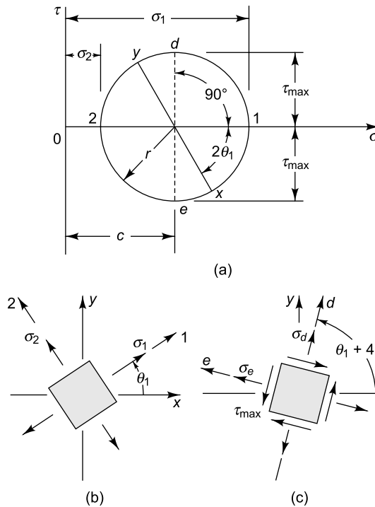
Fig. 4.19 (a) Principal stresses \sigma_1 and \sigma_2 and maximum shear stress \tau_{\max} indicated on Mohr's circle. (b) Element oriented along principal axes. (c) Element oriented along axes of maximum shear
