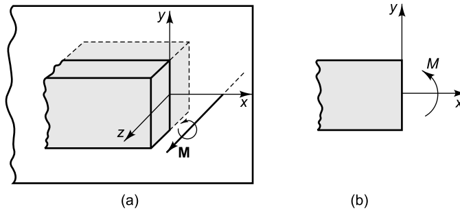
Fig. 1.11 Representation of a couple in a plane sketch
